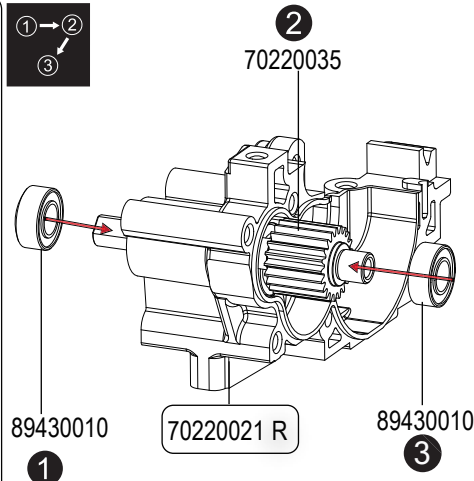
89430010 5x10x4mm Ball Bearing
